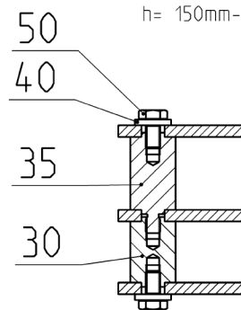
Schnitt/section B-B 1:2 h= 150mm-194mm
