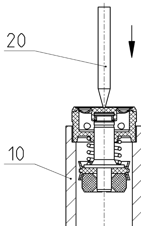
Demontage Teflonmembrane dismantling Teflon diaphragm
