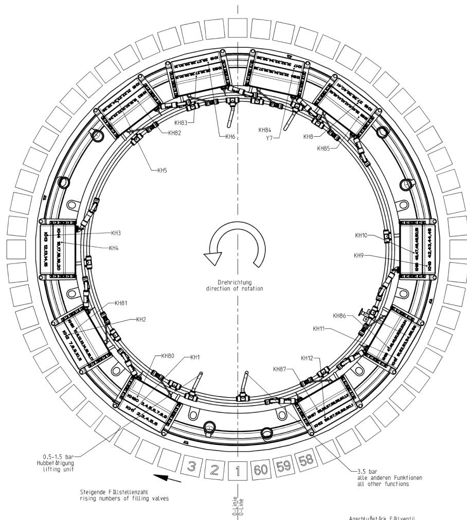
Füllventilinsel KH1-KH12 Solenoid valve module KH1-KH12
